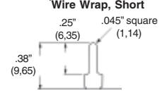
P 2 Printed Circuit and Wire Wrap, Short
