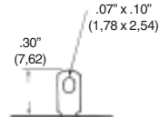
P Solder Eye (Standard)
