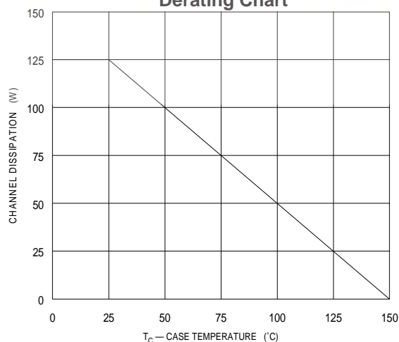
Derating Chart
