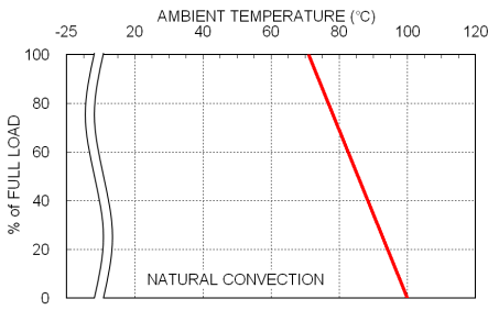
PMKC03-48S05 Derating Curve
