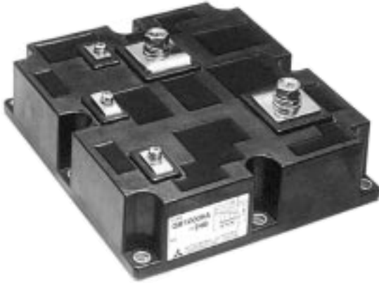
QM1000HA-24B
