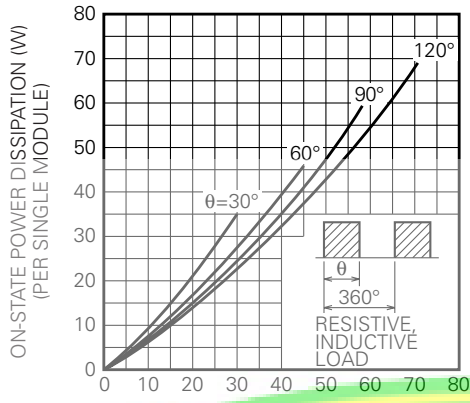
MAXIMUM ON-STATE POWER DISSIPATION (THREE PHASE FULLWAVE RECTIFIED)
