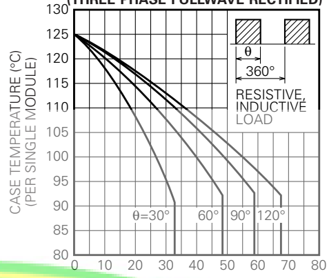
LIMITING VALUE OF THE DC OUTPUT CURRENT (THREE PHASE FULLWAVE RECTIFIED)
