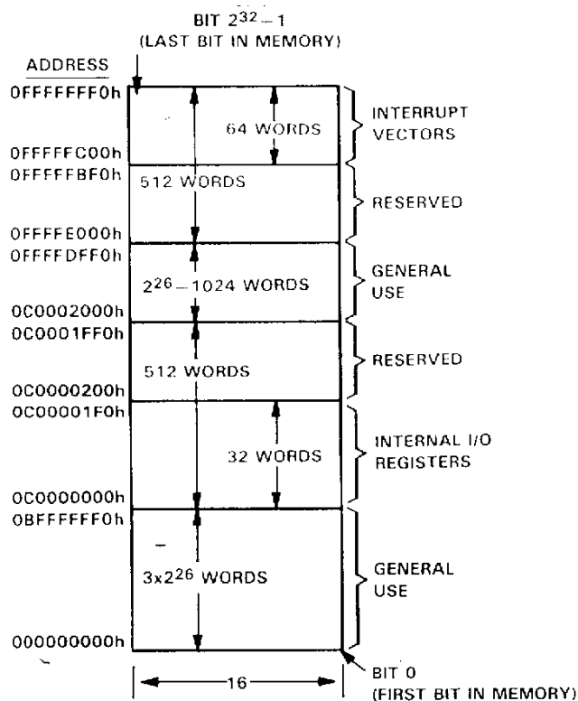
FIGURE 6. MEMORY MAP
