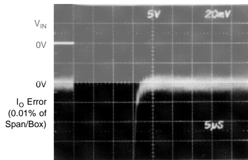
SETTLING TIME WITH POS V_{IN} STEP
