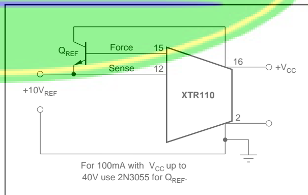
FIGURE 4. Increasing Reference Current Drive.
